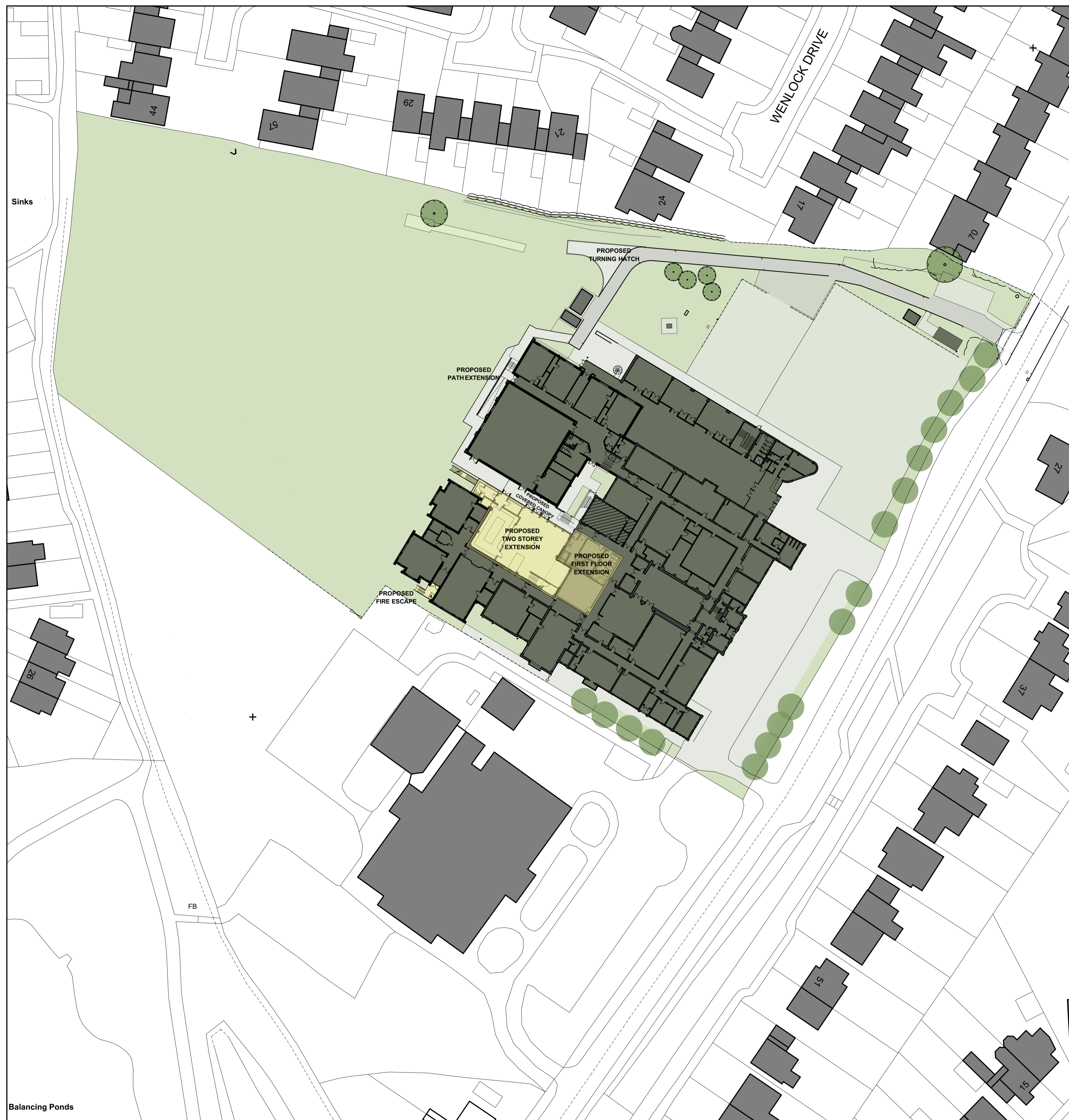
PROPOSED BLOCK PLAN Scale 1:500
